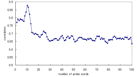
Figure 2: Number of probe words vs. correlation with KL scoring in the SN dataset.
